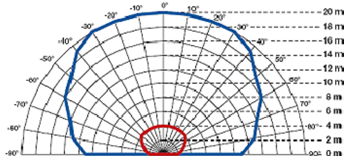
Detection zone of IS 2180-5, mounted at a height of 1.8 m, 20 m lens (blue = tangential walking direction, red = radial walking direction)
