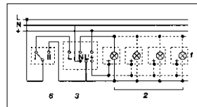
4. Connection to double-throw switch for permanent light and automatic operation Setting I: automatic operation Setting II: manual operation permanent light
